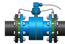
Non-conductive (plastic, lined) pipe
